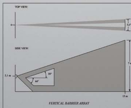
Figure 4. Distribution of beams and operating range of detector with vertical barrier lens (VB).
