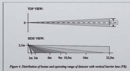
Figure 4. Distribution of beams and operating range of detector with vertical barrier lens (VB).
