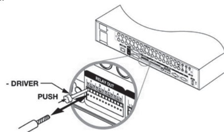
Figure 3.2.2 Inserting and Removing Wires
