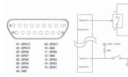
Figure 3.4.5 Digital Input/Output Connections
