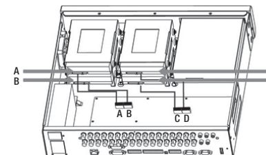
Figure 3.6.4 Connecting SATA cable
