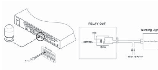
Figure 3.4.3 Relay Connections for a Warning Light
