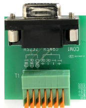
RS-485 terminal (NV-DVR1108/CD or NV-DVR1116/CD only)
