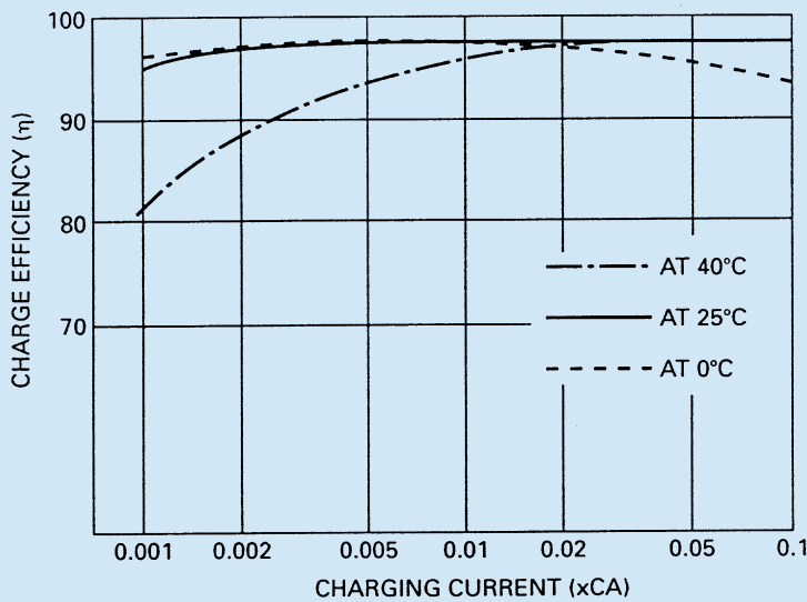
Figure 31. CHARGING EFFICIENCY
