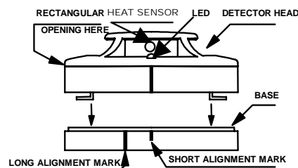
Fig. 2 Fitting detector head onto base
