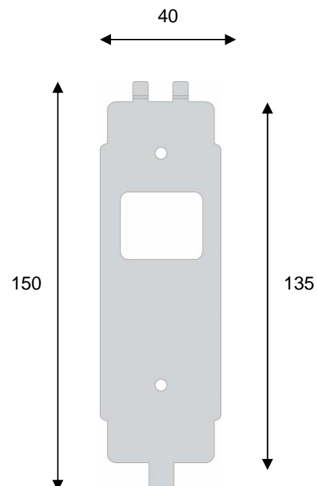
Metal Bracket
