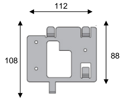
Bracket
