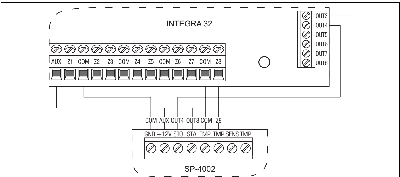
Fig. 21. Connection of siren with own power supply to low-current outputs (by the example of SP-4002 and INTEGRA 32 control panel). Audible signaling is triggered by OUT3 output, and optical signaling by OUT4 output (low-current outputs with normal polarization: when activated, they are shorted to ground). Z8 is programmed as tamper zone (NC type, function 9. 24H TAMPER).
