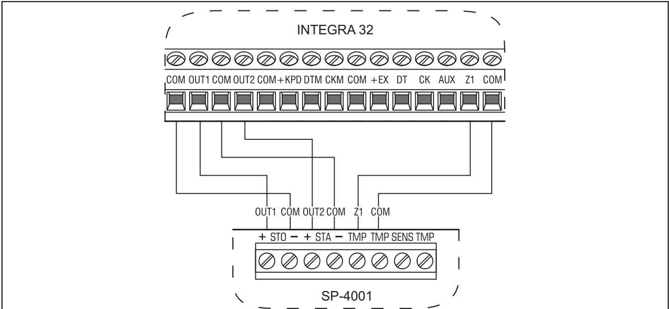
Fig. 20. Connection of siren without own power supply to high-current outputs (by the example of SP-4001 and INTEGRA 32 control panel). Optical signaling is triggered by OUT1 output, and audible signaling by OUT2 output (high-current outputs with normal polarization: when activated, +12 V voltage is supplied). Z1 is programmed as tamper zone (NC type, function 9. 24H TAMPER).
