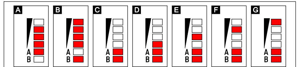
Fig. 3. Examples of LED indicated statuses. A (LED A is blinking, the other LEDs are lit up) – GPRS transmission is going on; signal level: 3. B (LED B is blinking, the other LEDs are lit up) – SMS message is being sent or converter is calling (CLIP test transmission); signal level: 4. C (LEDs are blinking) – logging into GSM network. D (LEDs are blinking) – logging into GSM network has failed; missing SIM card. E (LEDs are blinking) – logging into GSM network has failed; missing PIN code. F (LEDs are blinking) – logging into GSM network has failed; invalid PIN code. G (LEDs are blinking) – logging into GSM network has failed; SIM card has been blocked after three attempts to use an invalid PIN code (PUK code must be used to unblock the SIM card).
