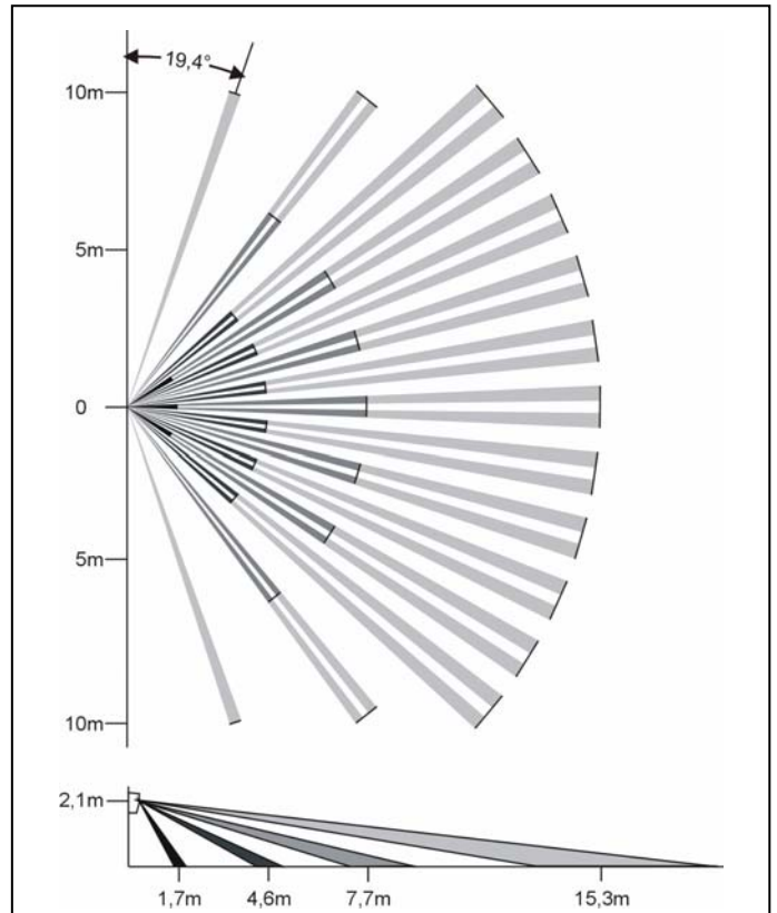
Fig. 5. Distribution of beams and operating range of detector with "EWA" lens.
