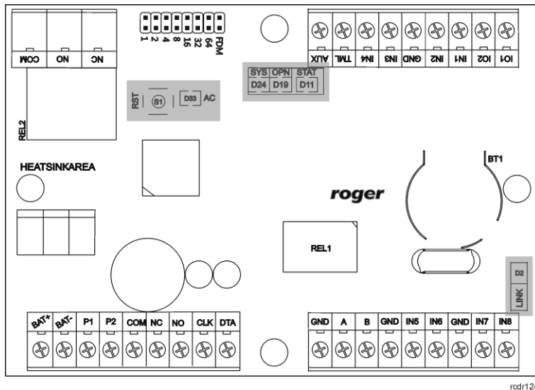
Fig. 3 LED indicators of CPR32-SE-BRD v3.0
