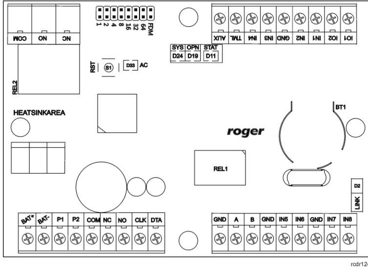
Fig. 1 CPR32-SE-BRD v3.0 network controller
