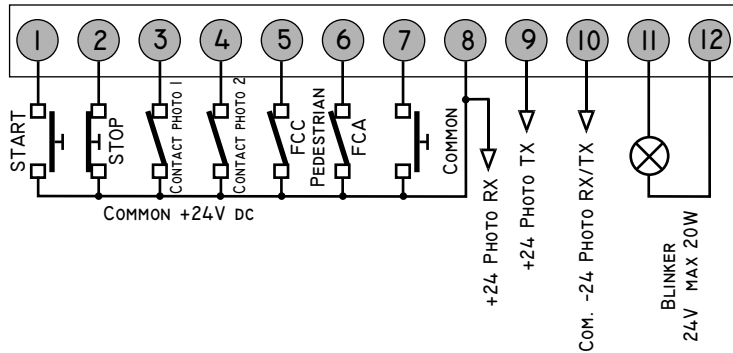
TERMINAL BLOCK 2
