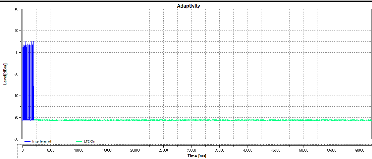
Adaptivity_LTE_11n HT20_5180
