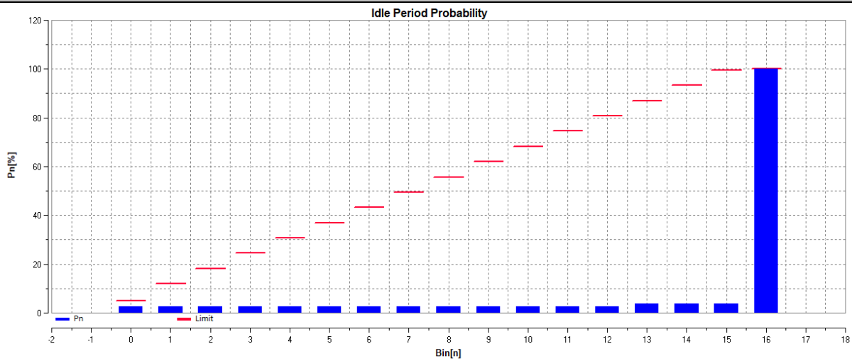
Adaptivity_Idle Period probability_11ac HT20_5180
