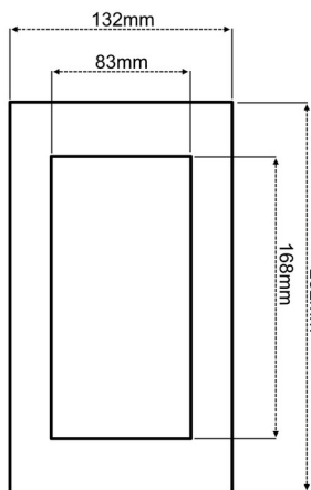
VDT-821/3x1 (3 modul)
