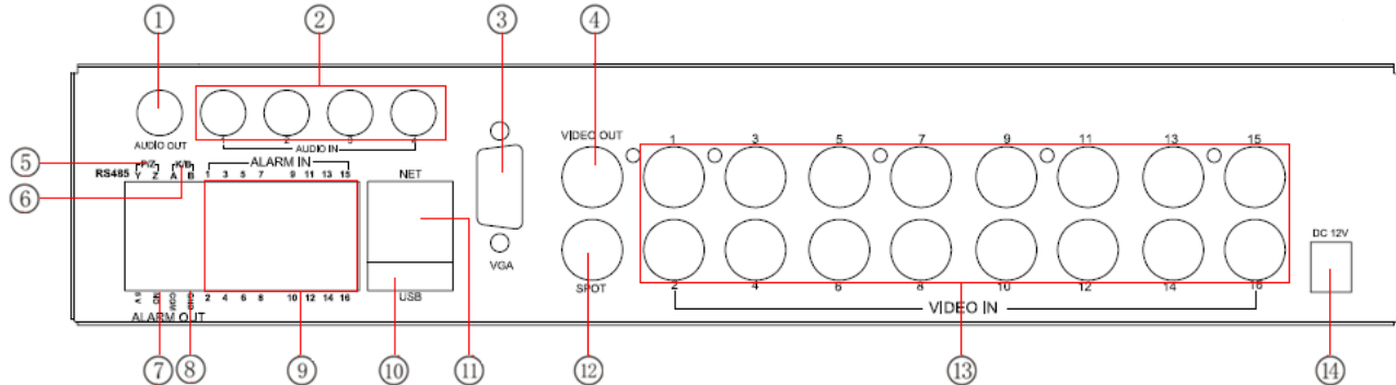
Fig 2.5 Rear Panel for 16-ch
