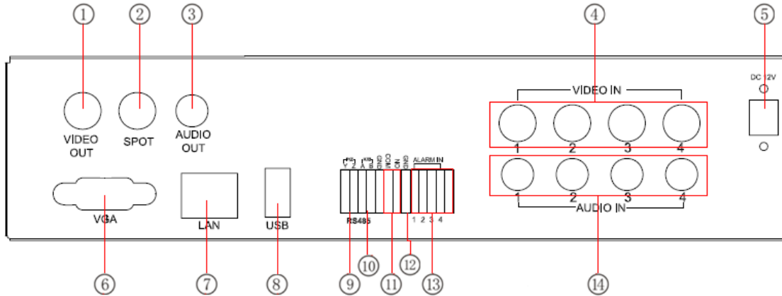
Fig 2.3 Rear Panel for 4-ch
