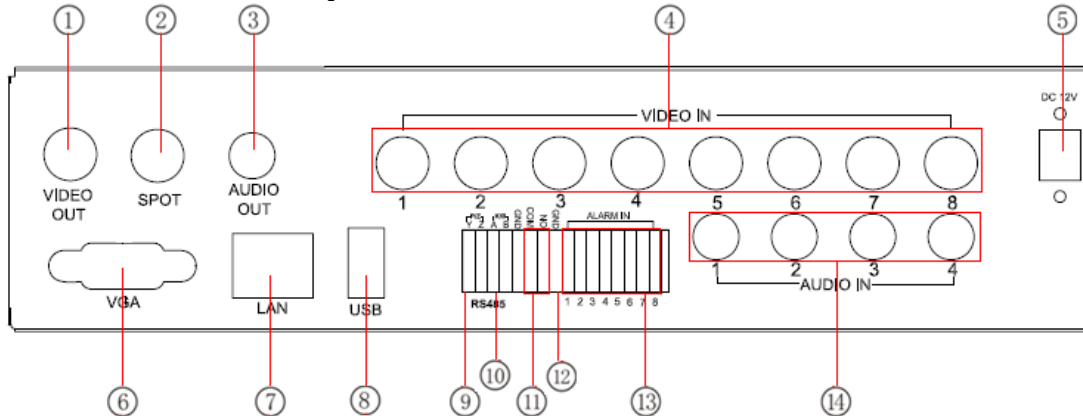
Fig 2.4 Rear Panel for 8-ch
