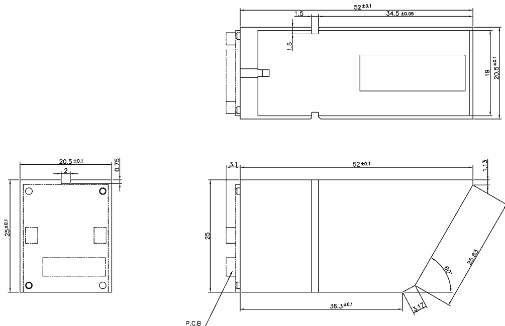
Figure 2 Sensor dimensions
