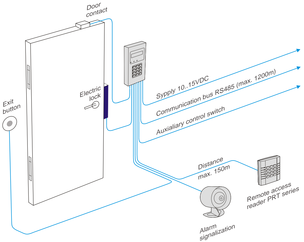
Typical connection diagram of access controller PR302LCD
